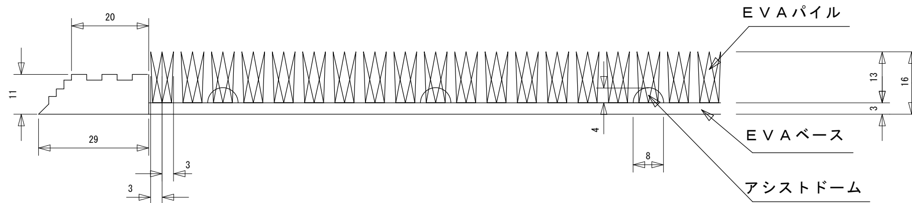
SECT A-A' (S=1/1)
