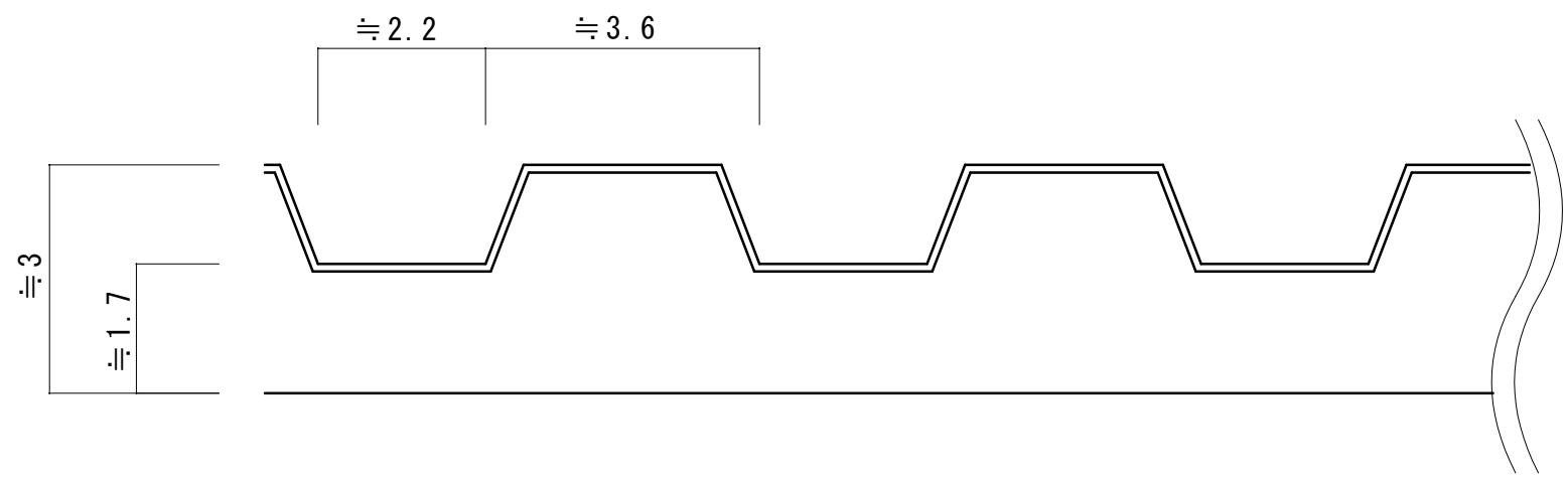
SECT A-A' (S=10/1)
