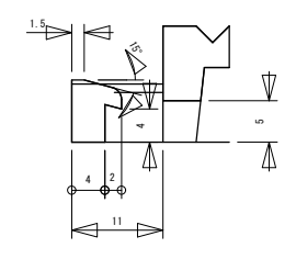
SECT D-D'
