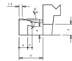
SECT D-D'
