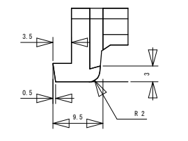
SECT E-E'
