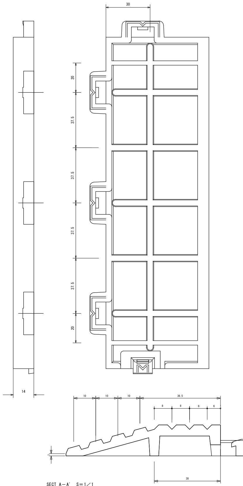
SECT A-A' S=1/1
