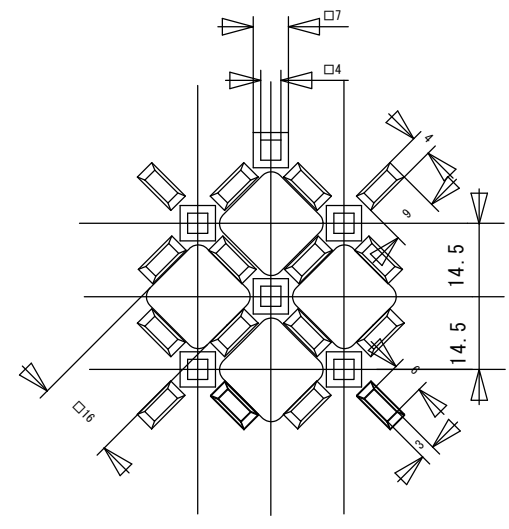
B部詳細 (S=2/3)
